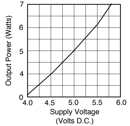
Max. Heater Power Available vs. Supply Voltage
